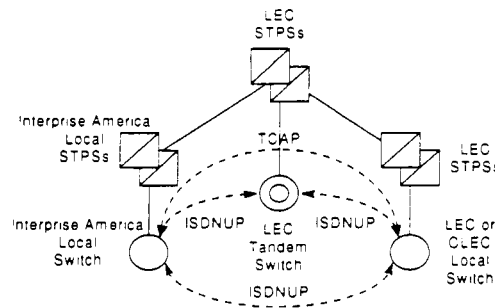
Figure 10. Interswitch TCAP Signaling for SS7 Network Interconnection
