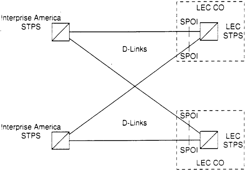
Figure 12. D-Link Interface
