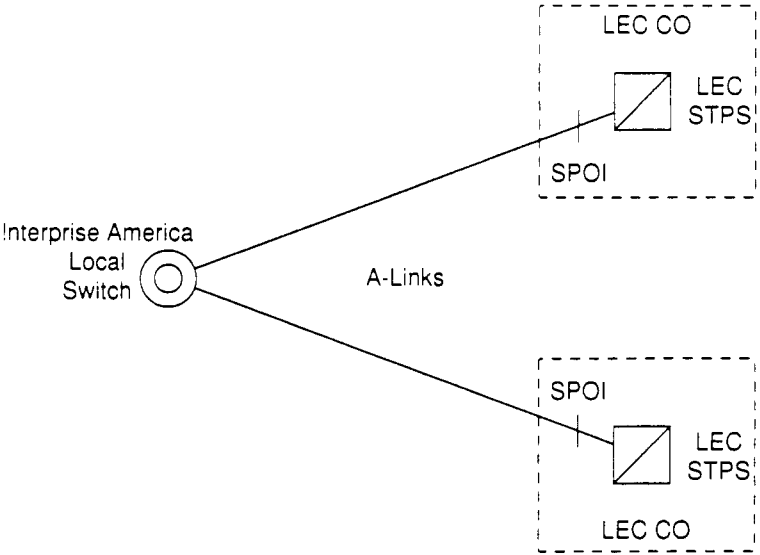
Figure 11. A-Link Interface
