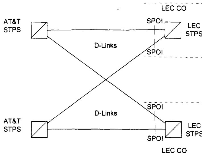
Figure 12. D-Link Interface
