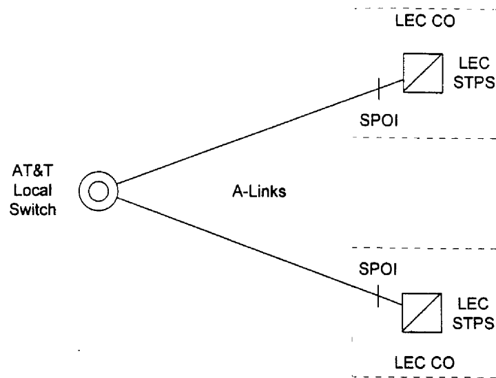
Figure 11. A-Link Interface
