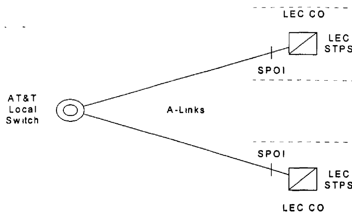
Figure 6. A-Link Interface
