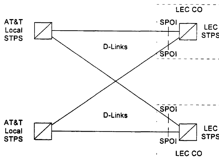
Figure 7. D-Link Interface
