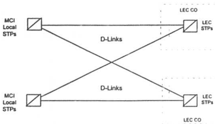
Figure 6. D-Link Interface
