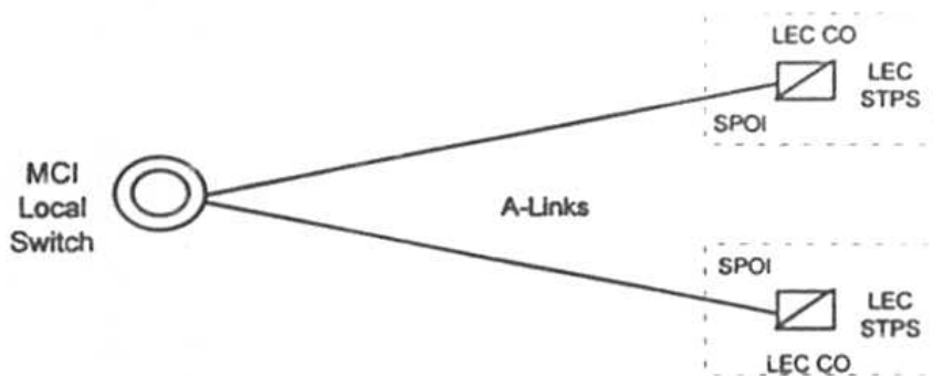
Figure 5. A-Link Interface
