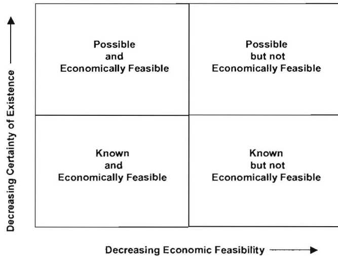
Figure 3-1: Conceptual Framework for Estimates of Fossil Fuel Resources
